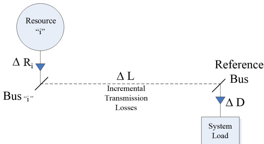
Figure 6: Incremental Transmission Losses
