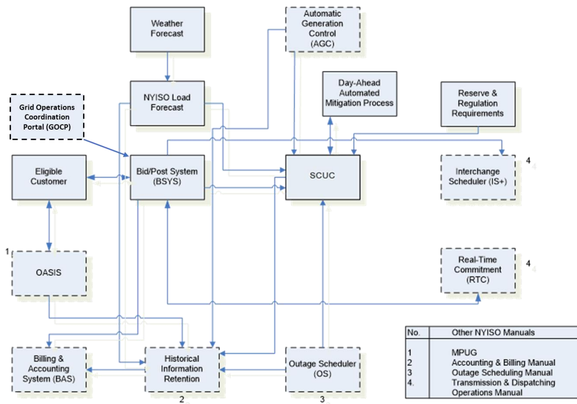
Figure 3: Day-Ahead Scheduling Data Flow
